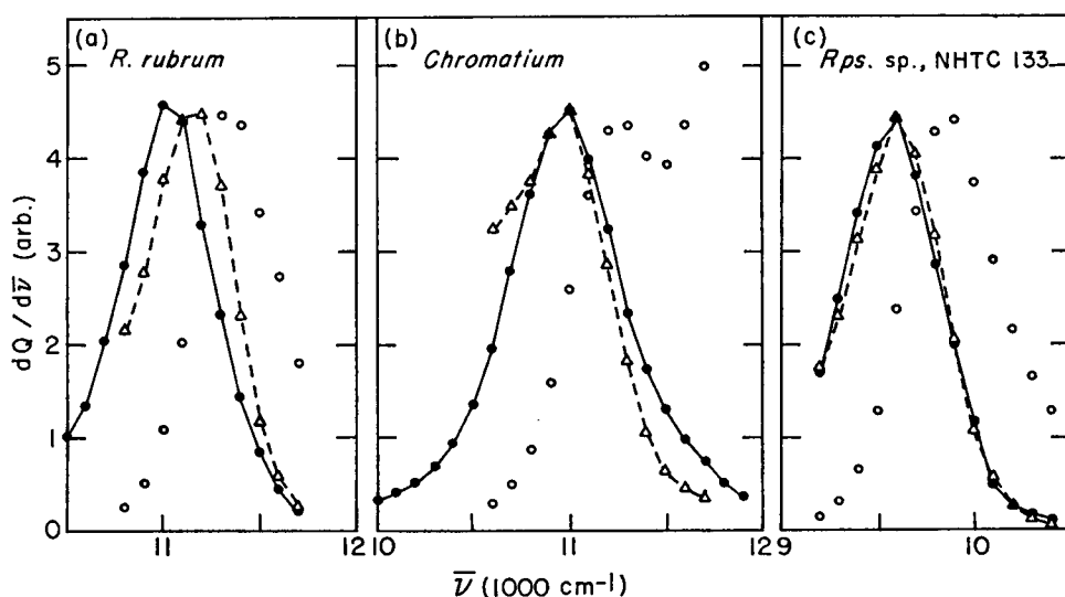
FIGURE 3 Comparison of calculated and experimental luminescence spectra of purple bacteria. Experimental absorption, ○, and luminescence, ●, data were taken at 100\text{ cm}^{-1} intervals from the curves of Olson and Stanton (1966) [luminescence data in (c) by Clayton] Solid line: experimental luminescence spectrum; dashed line: luminescence spectrum calculated from the absorption spectrum with the Planck factor for 295^\circ\text{K} .
